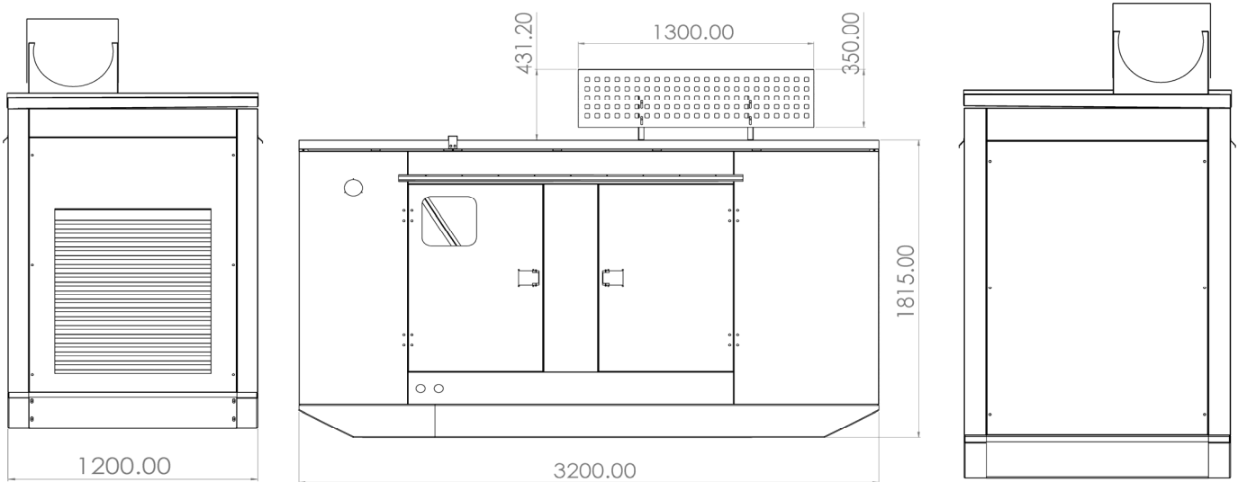
REAR VIEW
