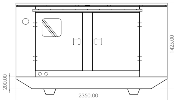
RHS VIEW
