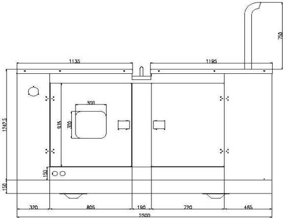
RHS VIEW
